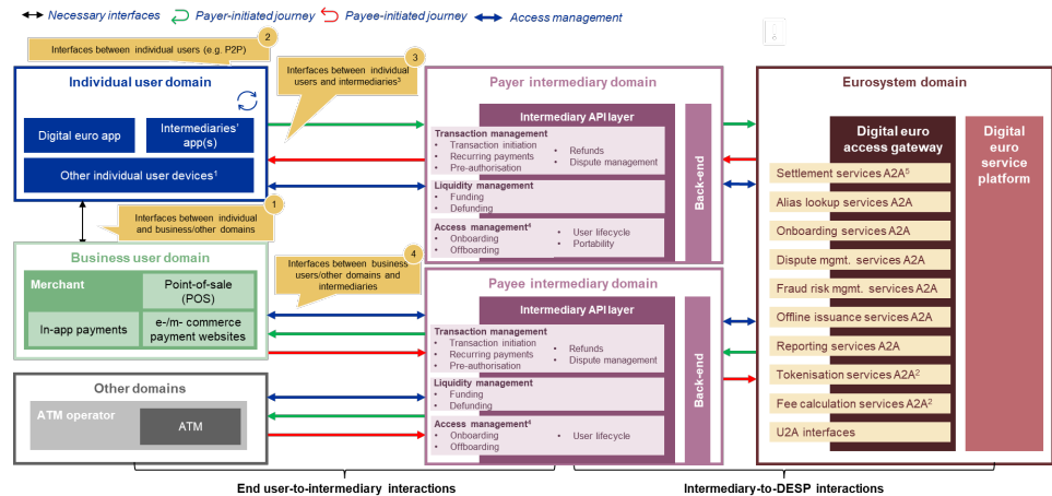
Figure 15 High-level architecture
